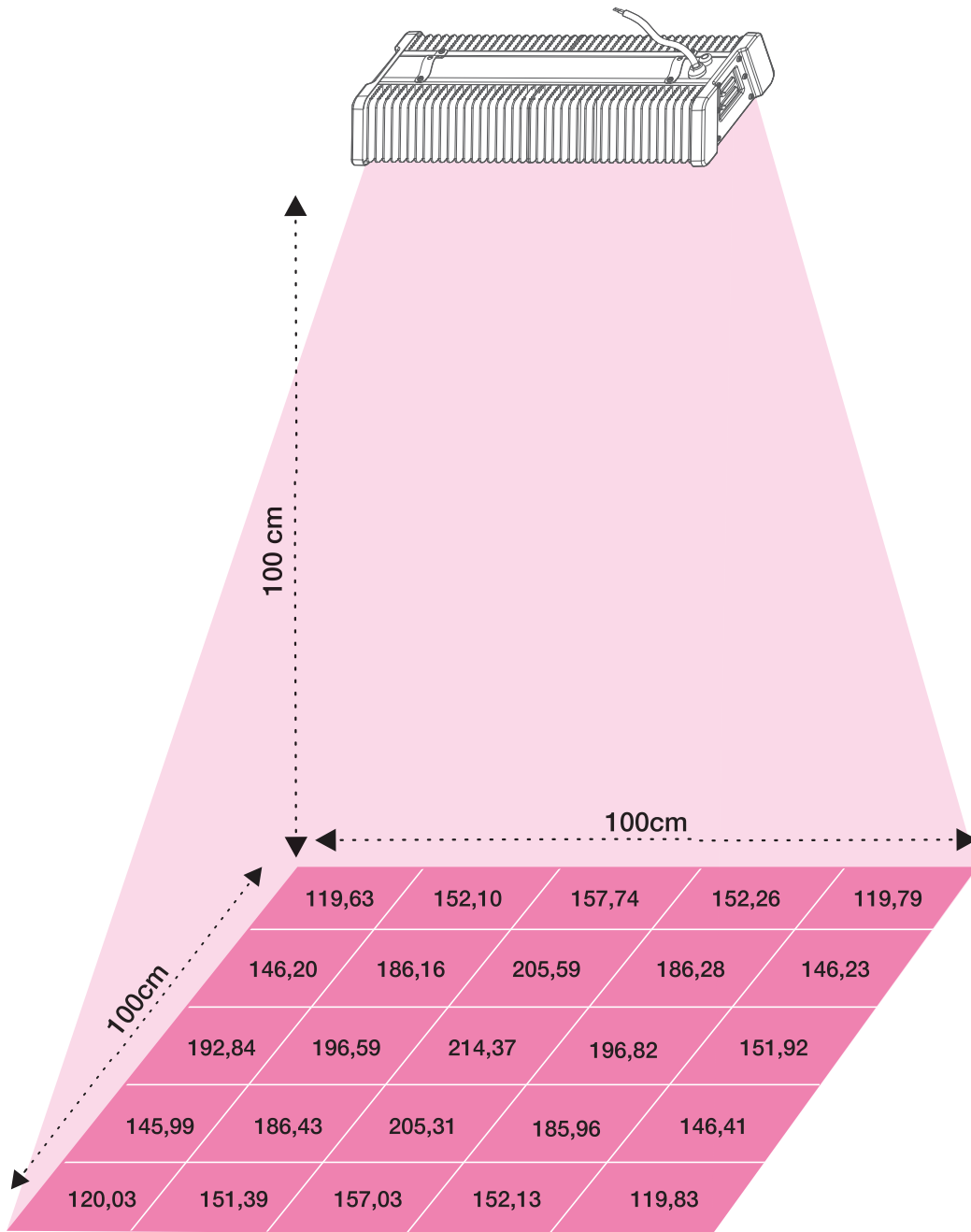
GS Sunray 300 / Dark Room / Height: 100cm [ All measurements are given in \mu\text{mol}/\text{m}^2/\text{s} ]
