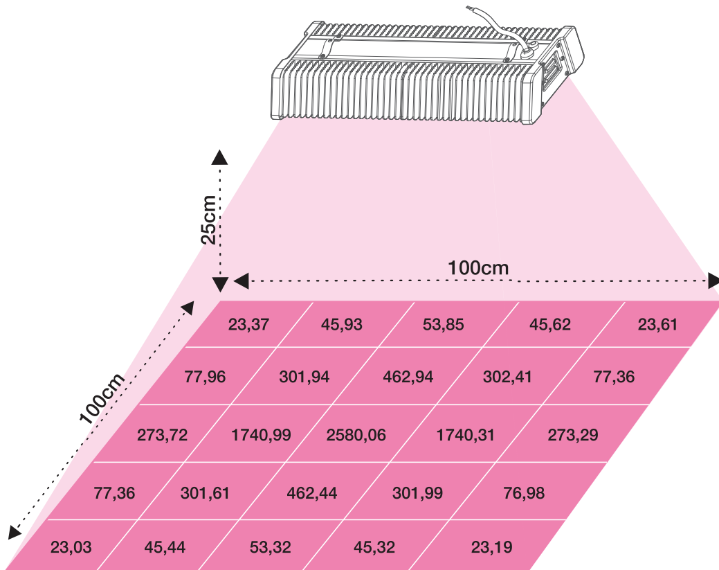
GS Sunray 300 / Dark Room / Height: 25cm [ All measurements are given in \mu\text{mol}/\text{m}^2/\text{s} ]
