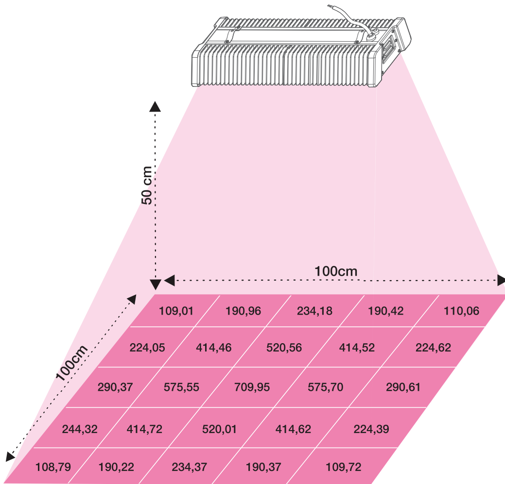
GS Sunray 300 / Dark Room / Height: 50cm [ All measurements are given in \mu\text{mol}/\text{m}^2/\text{s} ]
