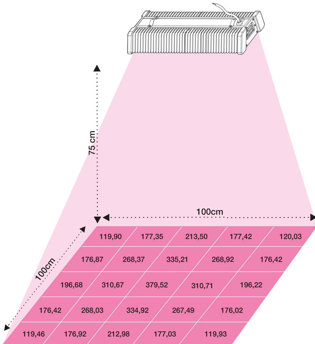
GS Sunray 300 / Dark Room / Height: 75cm [ All measurements are given in \mu\text{mol}/\text{m}^2/\text{s} ]
