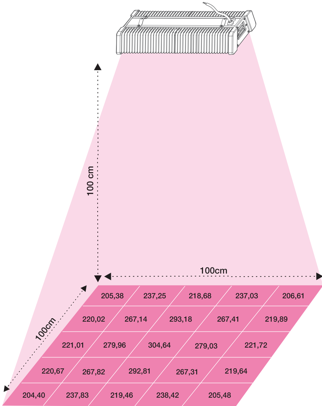
GS Sunray 300 / Tent with silver padding 200D / Height: 100cm [ All measurements are given in \mu\text{mol}/\text{m}^2/\text{s} ]
