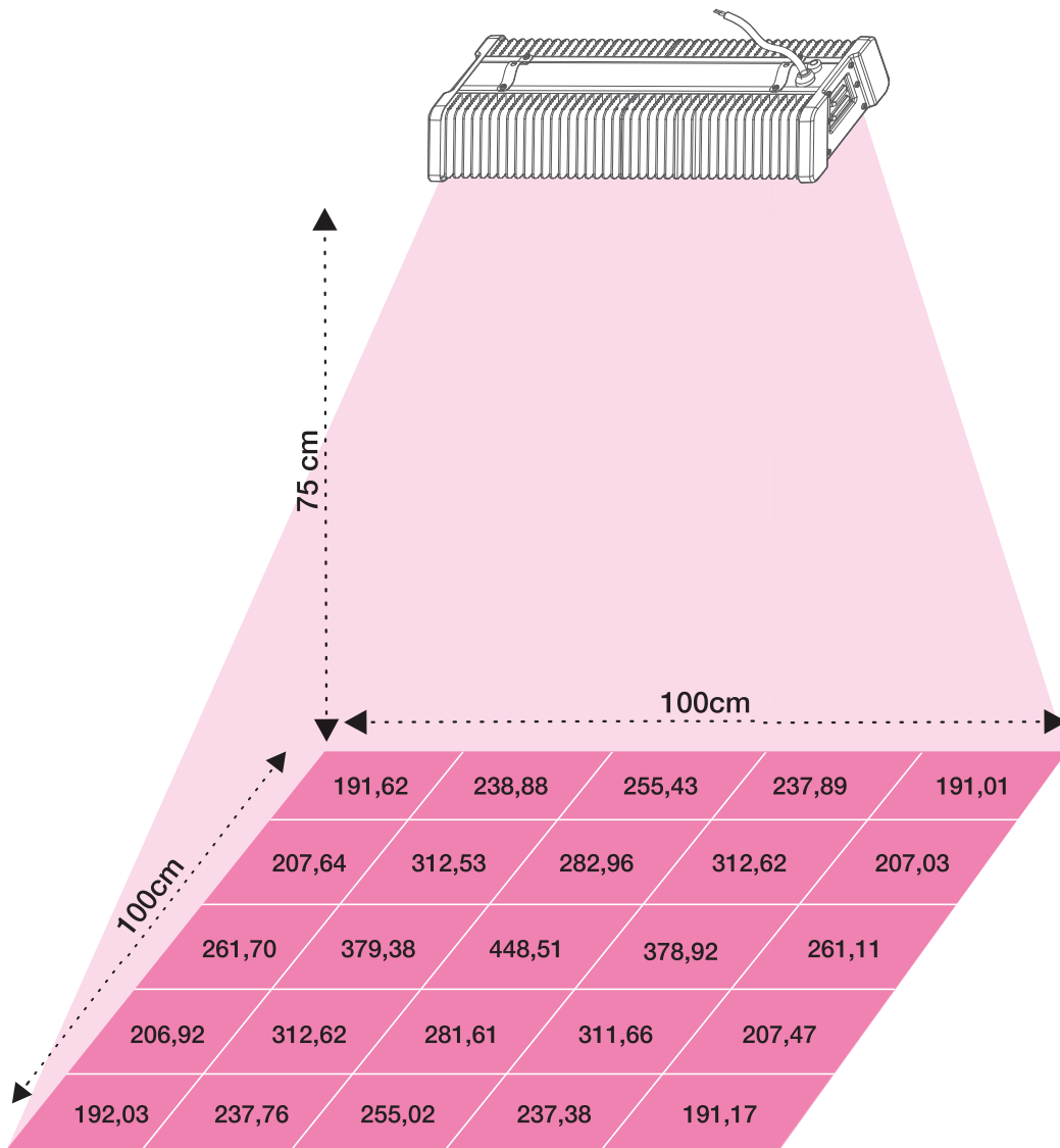
GS Sunray 300 / Tent with silver padding 200D / Height: 75cm [ All measurements are given in \mu\text{mol}/\text{m}^2/\text{s} ]
