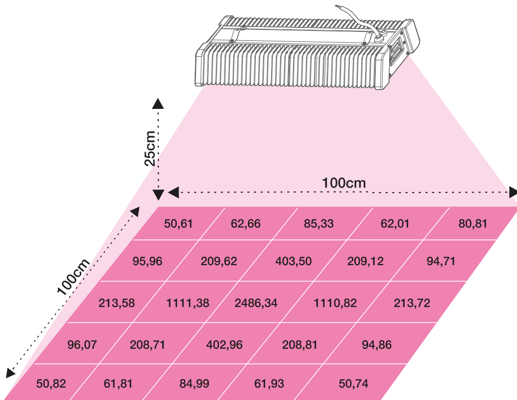
GS Sunray 300 / Tent with silver padding 200D / Height: 25cm [ All measurements are given in \mu\text{mol}/\text{m}^2/\text{s} ]
