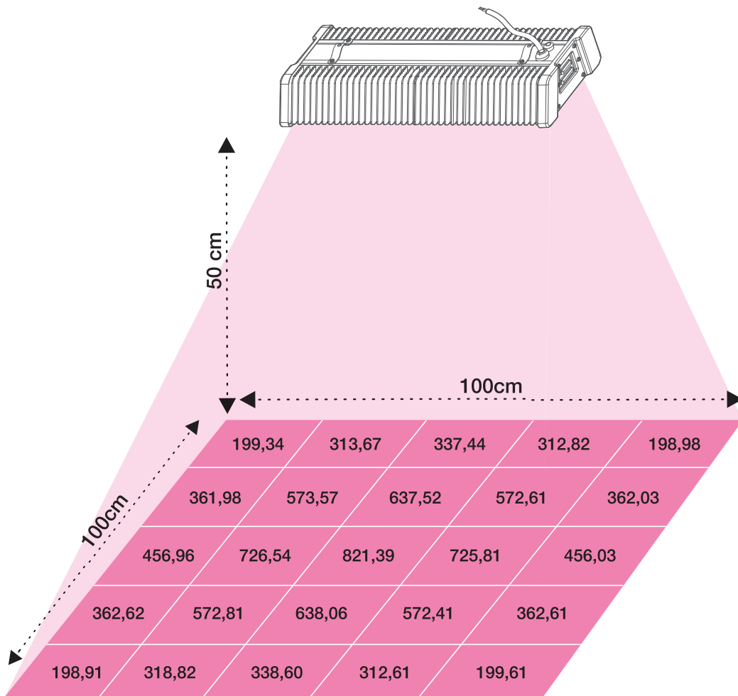
GS Sunray 300 / Tent with silver padding 200D / Height: 50cm [ All measurements are given in \mu\text{mol}/\text{m}^2/\text{s} ]
