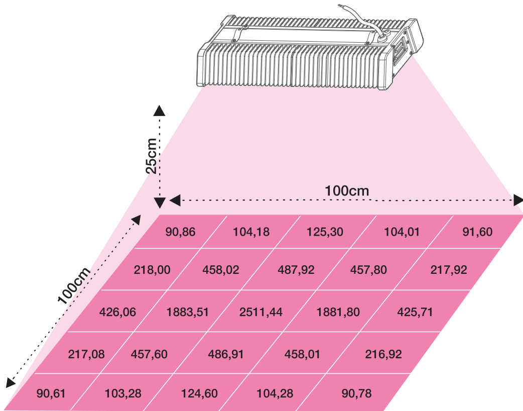
GS Sunray 300 / Growspec tent with white padding 1680D / Height: 25cm [ All measurements are given in \mu\text{mol}/\text{m}^2/\text{s} ]
